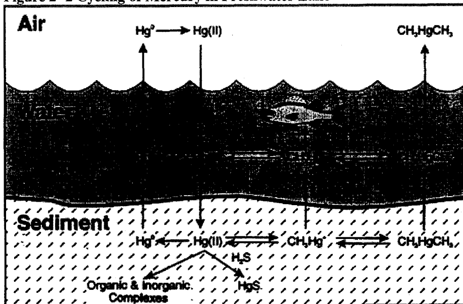
Figure 2 -2 Cycling of Mercury in Freshwater Lake
